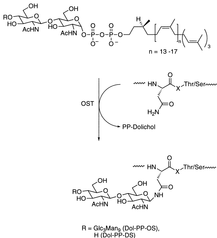
Figure 1. OST-catalyzed N -linked glycoprotein synthesis.
